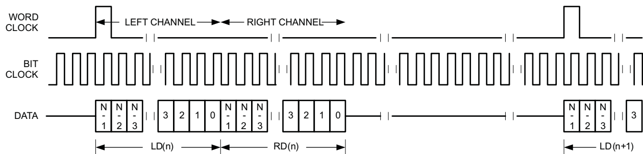
Figure 5-30. Timing Diagram for DSP Mode With Offset = 0 and Bit Clock Inverted
