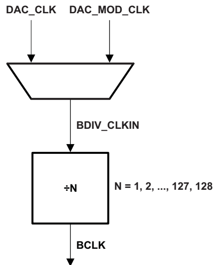
Figure 5-18. BCLK Output Options
